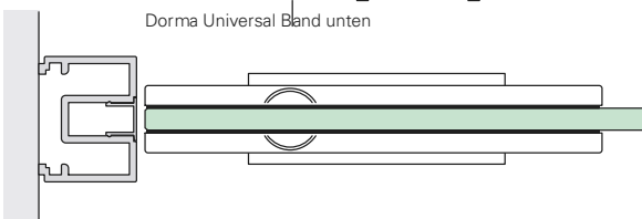
Grundriss Dorma Universal Band
