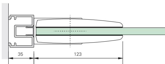
Dorma Tensor Band
