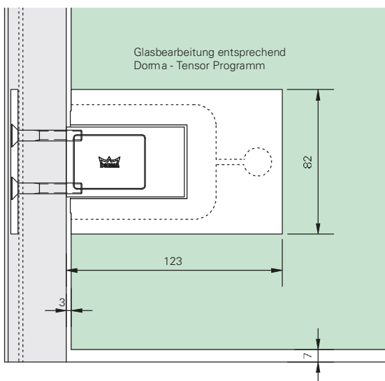
Dorma Tensor Band
