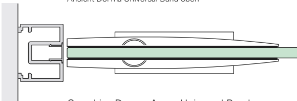
Grundriss Dorma Arcos Universal Band
